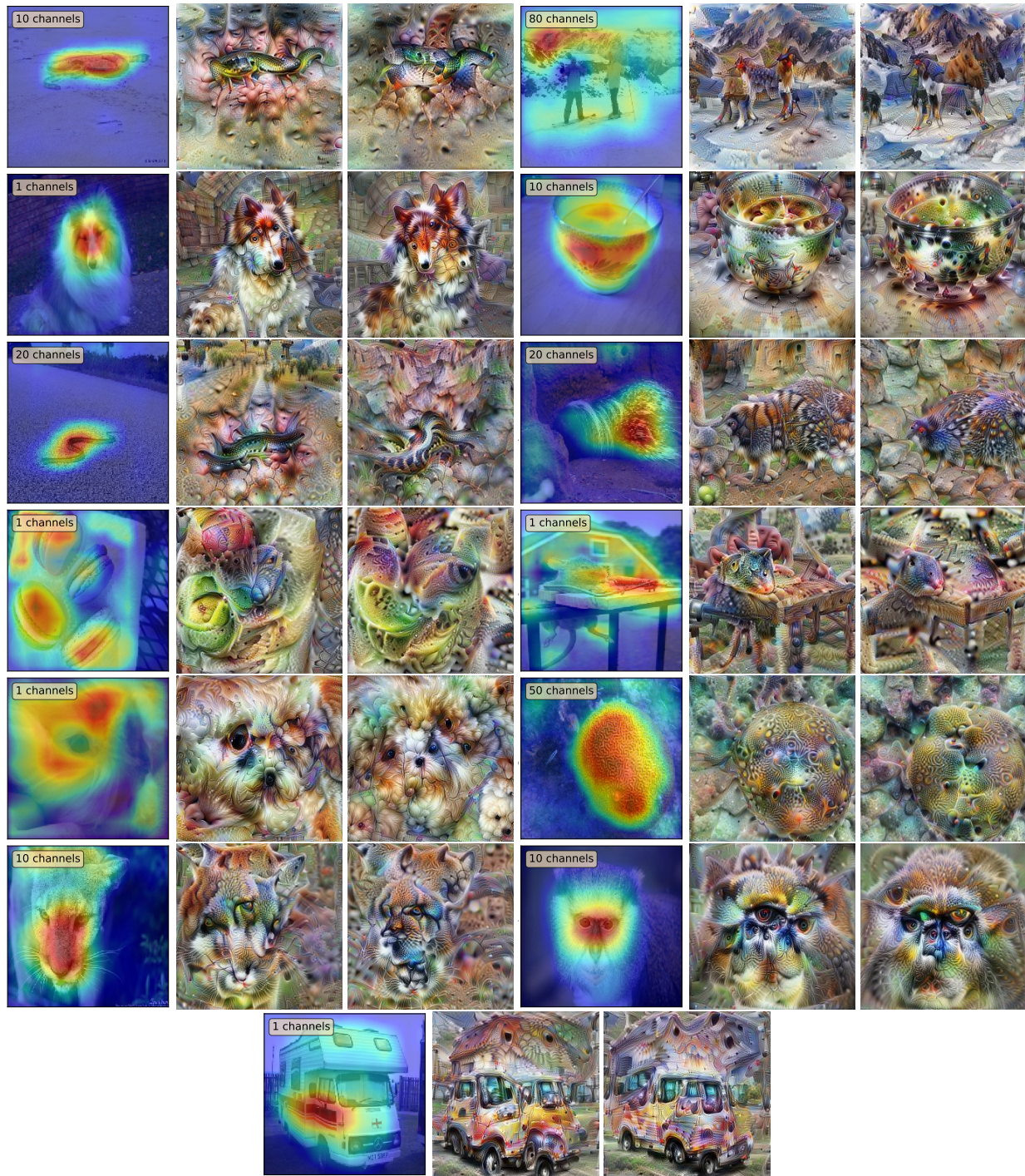
Figure 16: Per-instance channel attribution visualization (1-14). Left: input image overlaid with channel saliency map (see eq. 13 in main paper). Middle: feature inversion of original activation tensor. Right: feature inversion of activation tensor perturbed by optimal channel mask m_{a^*} . By comparing the difference in feature inversions between un-perturbed (middle) and perturbed activations (right), we can identify the salient features that our method highlights. Notable examples are the crib (3rd row, left) and snakes (1st row, left and 3rd row, right). These are visualizations for the ImageNet validation images 1-14.
