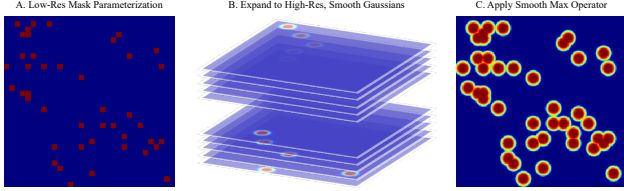
Figure 2: Generating smooth masks. a. We first define a low resolution parameterization mask, \tilde{\mathbf{m}} \in [0, 1]^{H \times W} (shown as a binary mask in this illustration). b. We then represent each location in \tilde{\mathbf{m}} as a high resolution, smooth Gaussian, weighted by the value in \tilde{\mathbf{m}} . c. Finally, we apply the smooth max operator across all locations to get our final mask.
