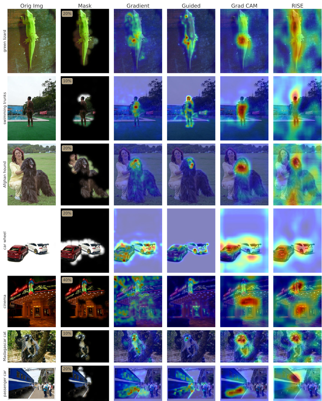
Figure 3: Comparison with other visualization methods.
