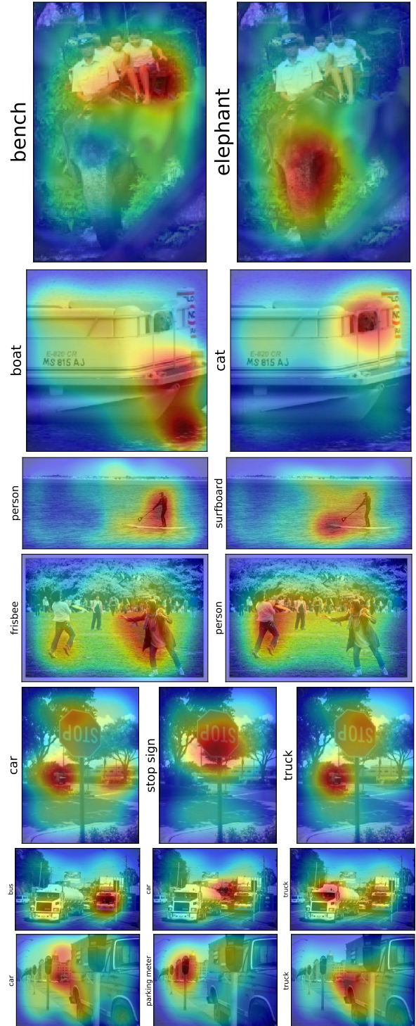
Figure 15: Pointing Examples from COCO. The overlaid visualization is the average mask after Gaussian smoothing ( \sigma = 20 ).
