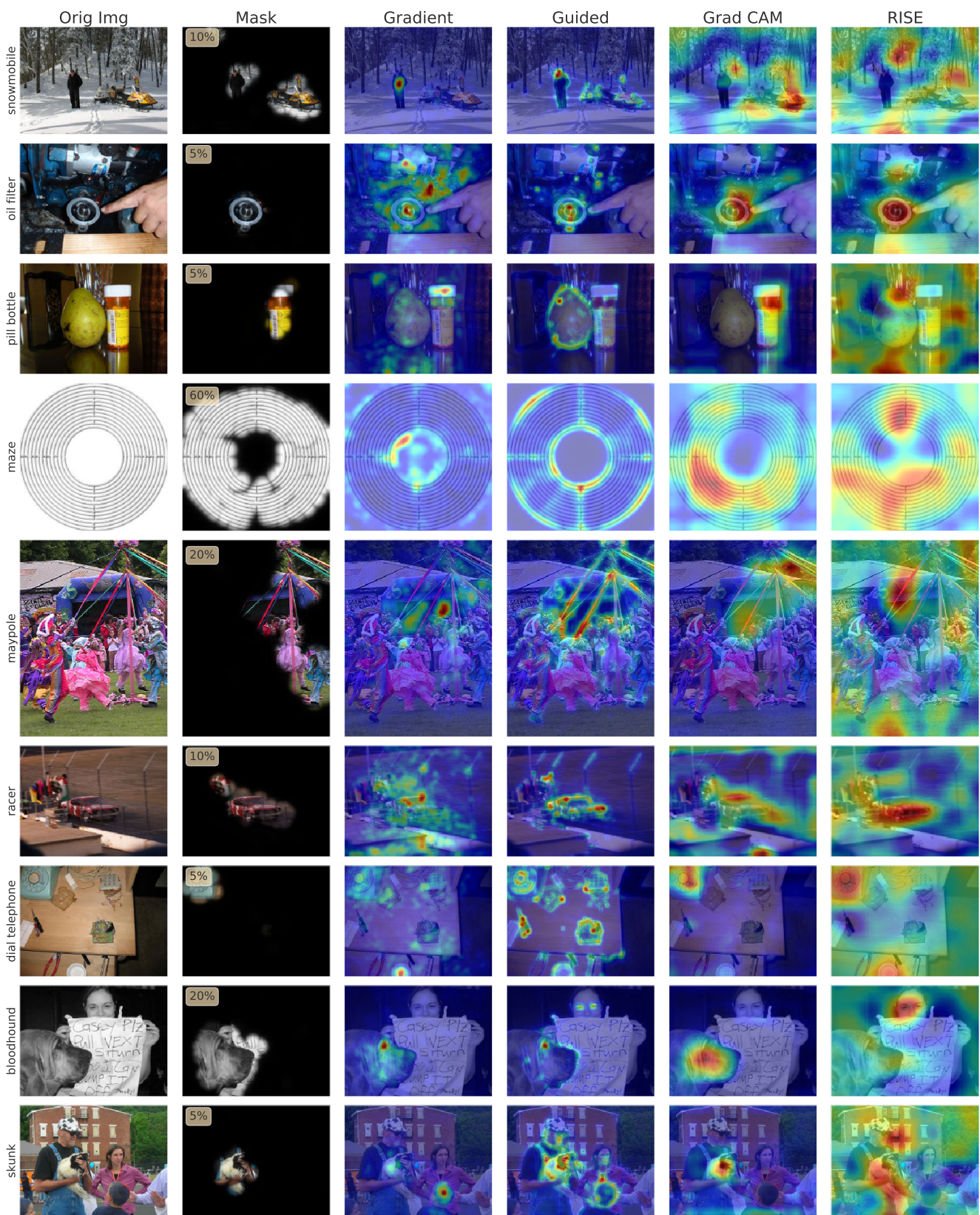
Figure 4: Comparison with other visualization methods (more examples).
