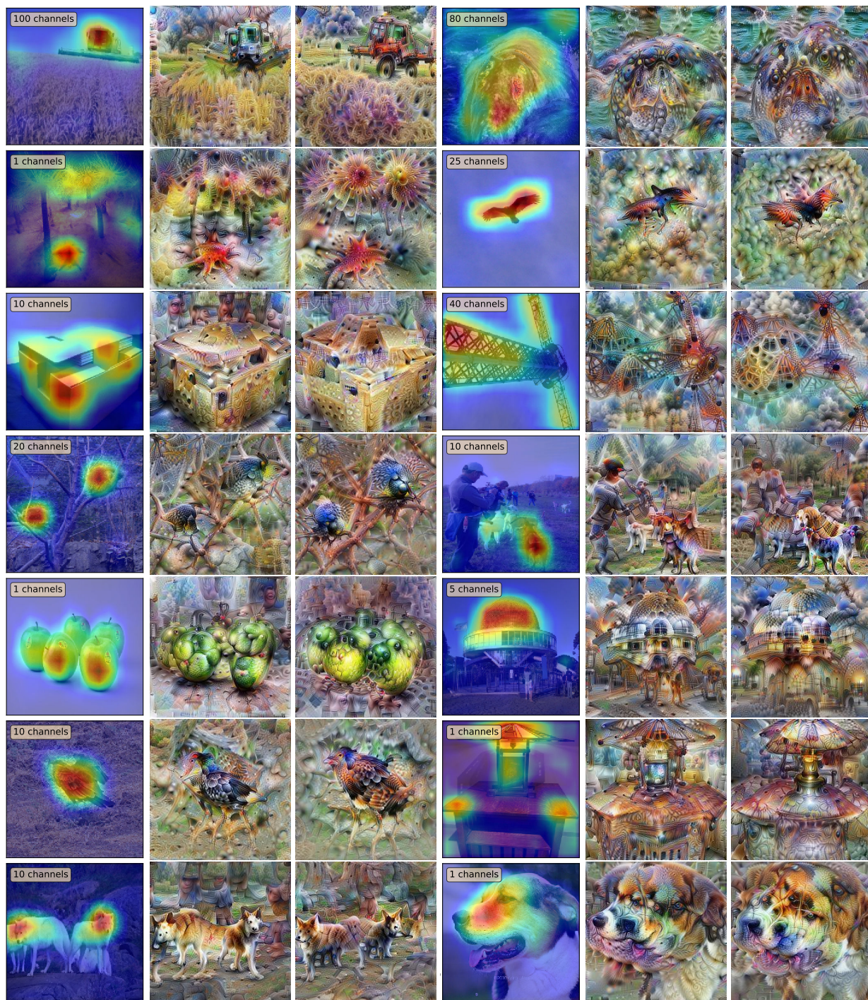
Figure 17: Per-instance channel attribution visualization (15-28). Left: input image overlaid with channel saliency map. Middle: feature inversion of original activation tensor. Right: feature inversion of activation tensor perturbed by optimal channel mask m_{a^*} . Notable examples are the harvester (1st row, left), porcupines (4th row, left), and the bird (2nd to last row, left). These are visualizations for the ImageNet validation images 15-28.
