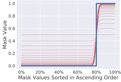
Figure 1: Area constraint. The blue line is the reference vector \mathbf{r}_a representing the target area a as a proportion of “on” versus “off” pixels (here a = 20\% ). The red dotted lines represent mask values in ascending, sorted order, \text{vecsort}(\mathbf{m}) , at different points of the optimization, starting by initializing \mathbf{m} to 1/2 . Over time, the optimization encourages the mask to match the target area. Even in the limit, there is a slight difference between \mathbf{r}_a as \mathbf{m} as the latter is forced to be smooth at the boundaries; this has the further beneficial effect of minimizing the boundary length, encouraging more compact masks.
